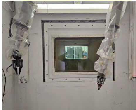
Alaron's shielded hot cell with telemanipulator arms.
