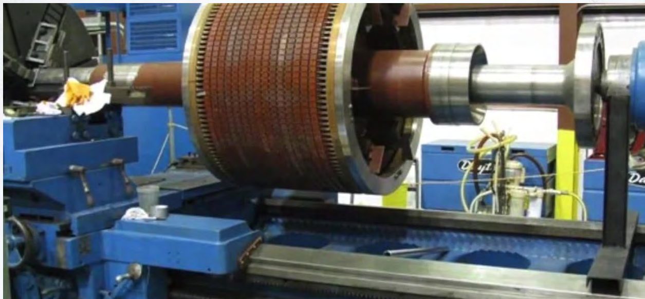
A motor rotor on the rebuild stand at the WCS Alaron Facility.
