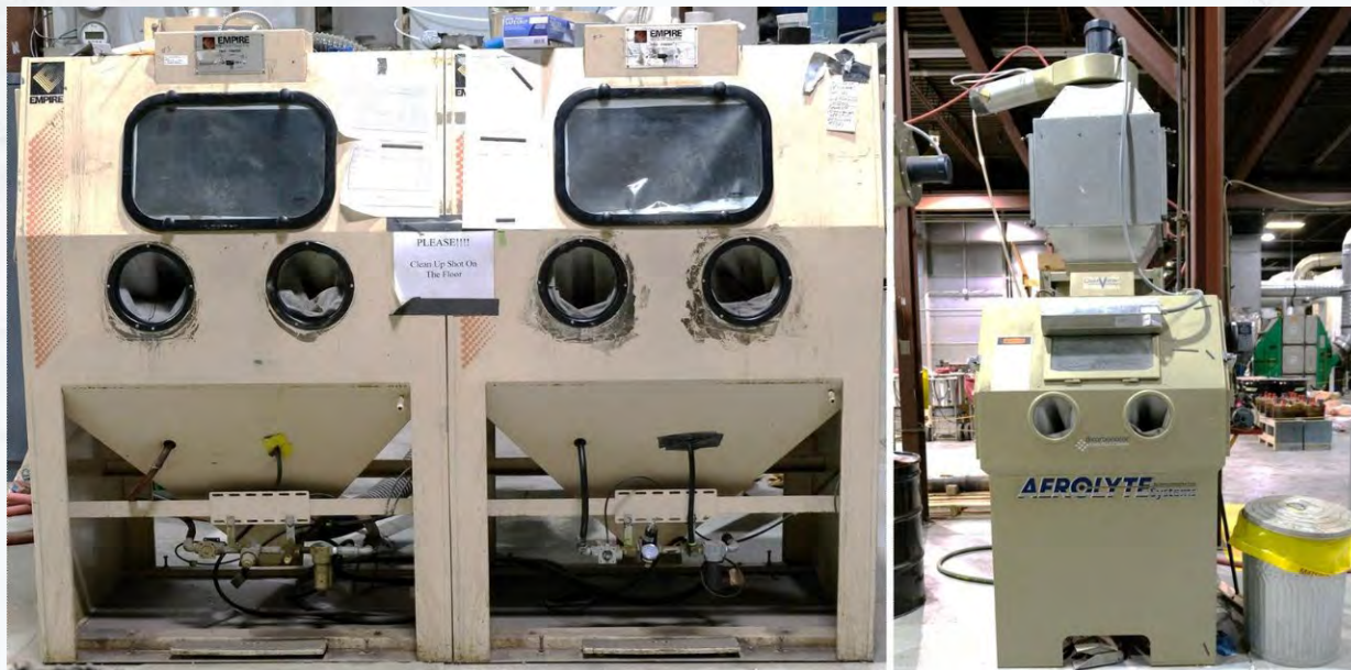
A WCS Alaron glove box used for contained handling of small components.
